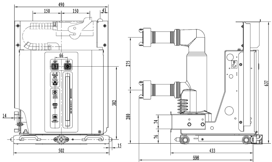
6.1 Handcart type circuit breaker (phase distance 150 mm) outline drawings:
