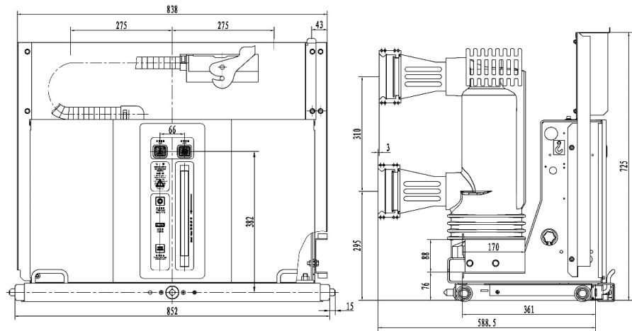
6.3 Handcart type circuit breaker (phase distance 275 mm) outline drawings
