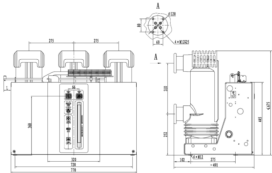
6.6 Fixed type circuit breaker (phase distance 275 mm) outline drawings:
