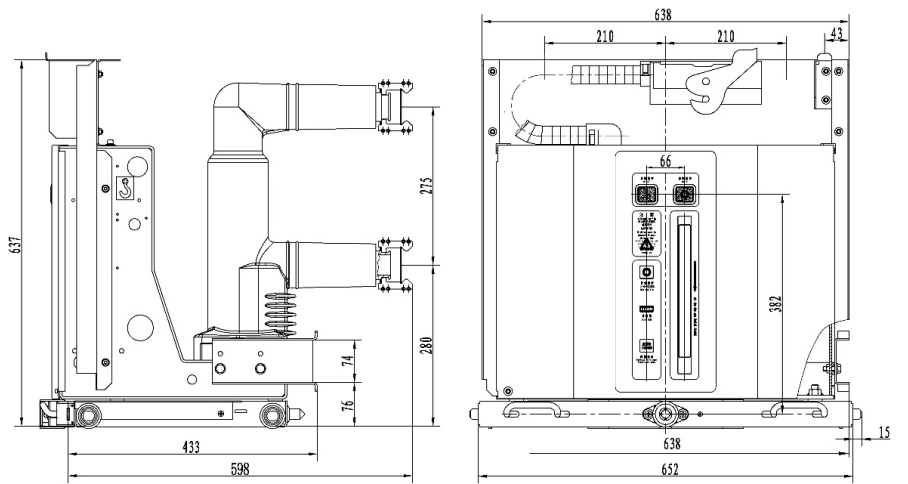
6.2 Handcart type circuit breaker (phase distance 210 mm) outline drawings
