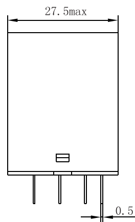
Left view
