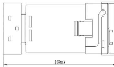
Outline and installation dimension for TGJS1 series product
