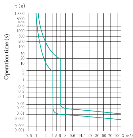
B(Ii=5In) type: Thermal / Electromagnetic characteristics protection curve
