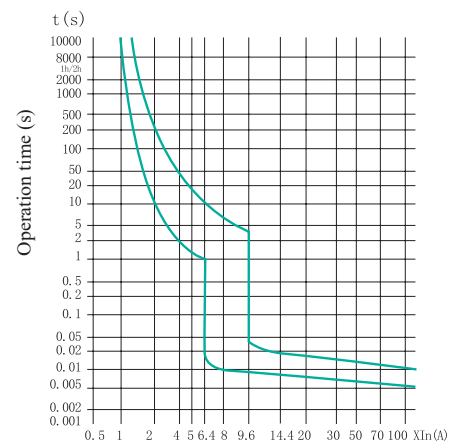
C(Ii=8In) type: Thermal / Electromagnetic characteristics protection curve
