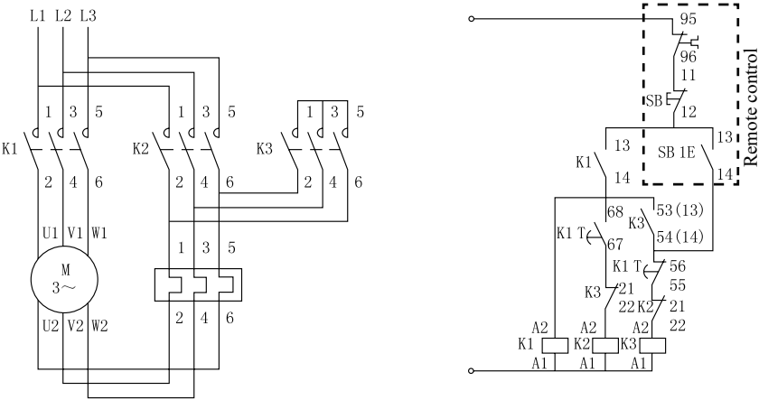
5.1 Start-delta starting wiring diagram
