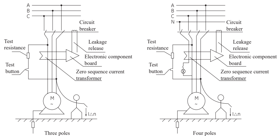
Fig. 1 Working principle
