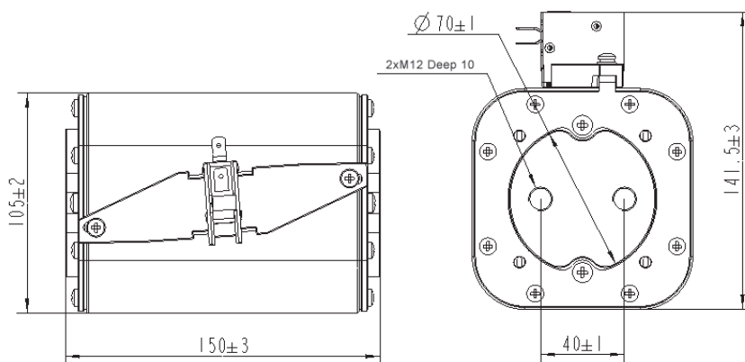
With micro switches
