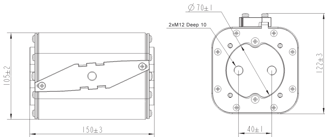
With indicator (without micro switches)
