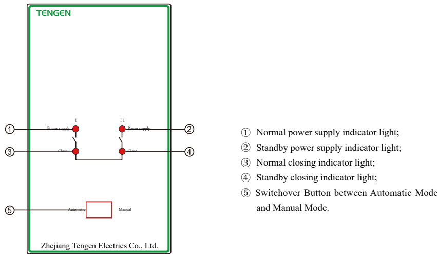
125-800 frame A type controller
