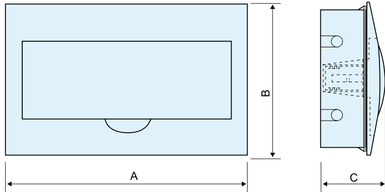
Dimension drawings of concealed box
